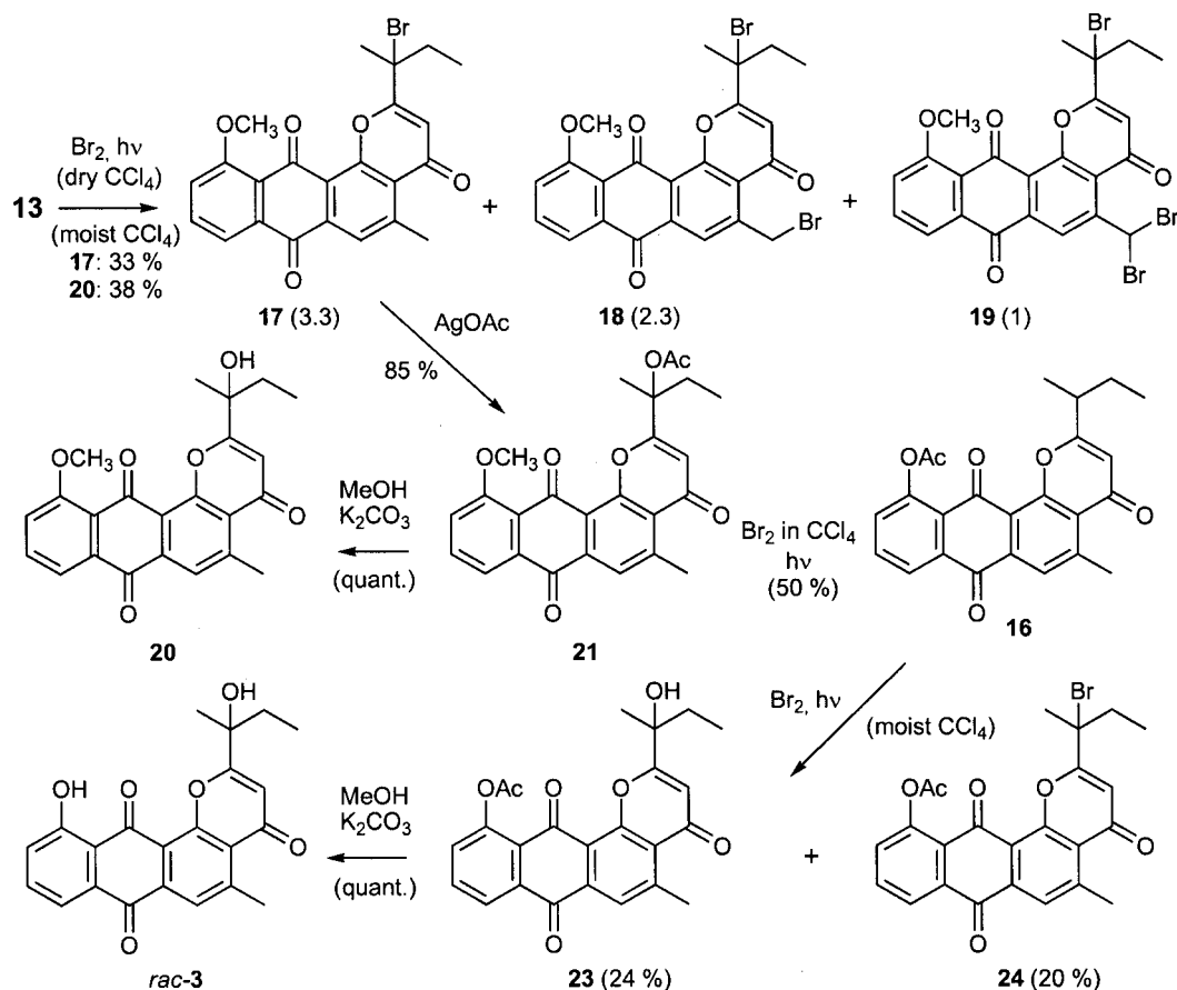
Scheme 2. Synthesis of rac - 20 and the natural product rac - 3 by transesterification in basic methanol of 21 and 23 , respectively.
