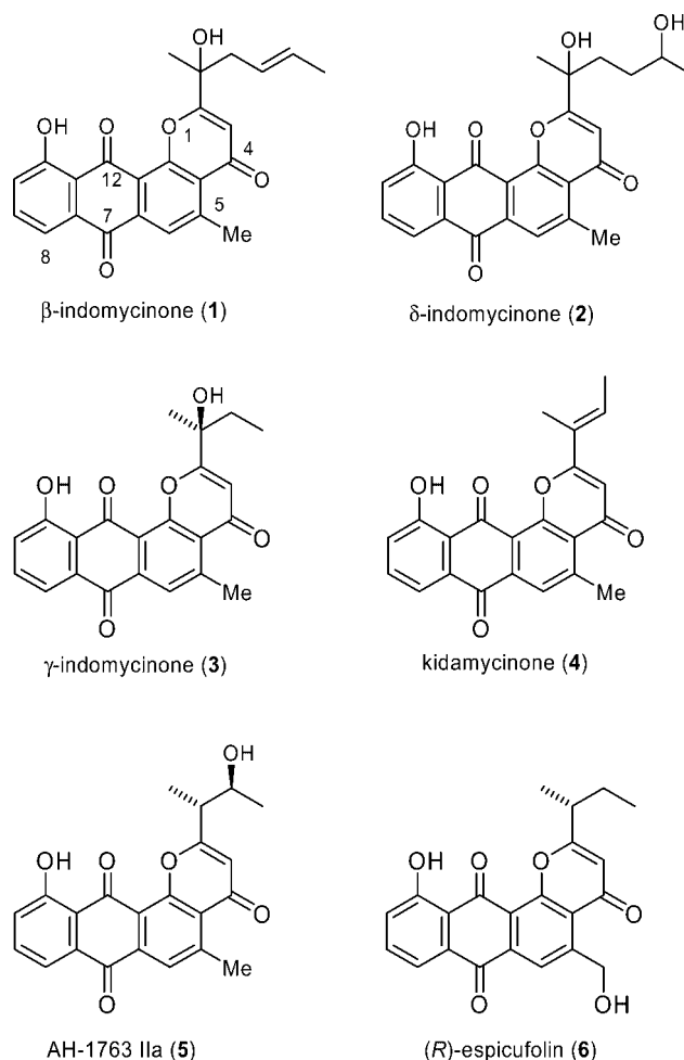
Figure 1. Representative anthrapyranone antibiotics with C-6 or C-4 side chains.
