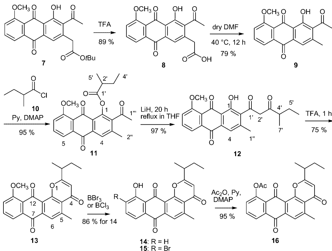
Scheme 1. Synthesis of the basic anthrapyranone skeletons 13 – 16 by Baker–Venkataraman rearrangement of 12 .
